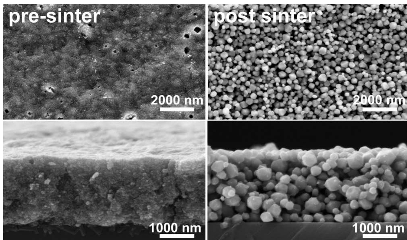
Figure 3. Top- and side-view SEM images of a pyrite NC film on a glass substrate before and after sintering at 540 °C in sulfur vapor.
